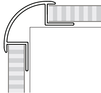
ACP81679 Corner Post Shallow Fit
