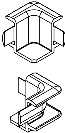
ACP1434 Internal Corner
